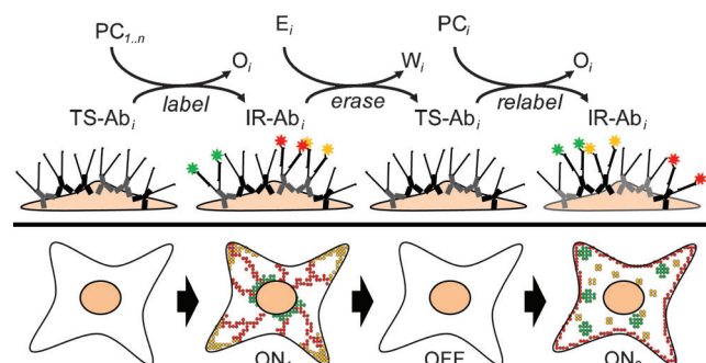
Figure 1. Multiplexed (multicolor) and reiterative (multiple cycles) in situ immunofluorescence labeling of proteins within fixed cells by using dynamic DNA complexes. Proteins are labeled by antibodies conjugated to a ssDNA targeting strand and a probe complex carrying a quencher domain (qd). The resulting labeling (ON 1 state) can be erased (OFF state) by incubation with an eraser complex, and proteins (the same or different ones) can be labeled again with other probe complexes (ON 2 state).
